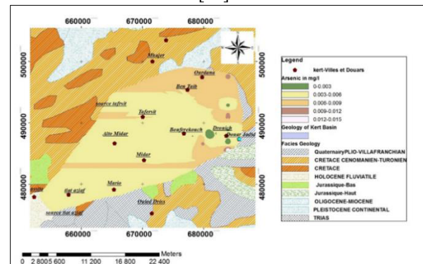
Fig. 6. Arsenic distribution in Kert groundwater.
