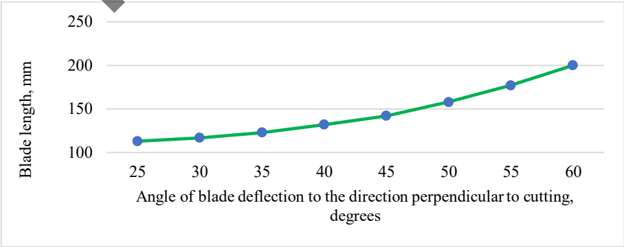
Fig. 10. Dependence of the blade length on the blade deflection angle in relation to the direction perpendicular to the cutting.
