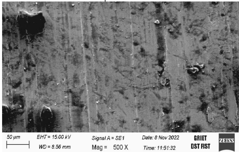
Fig.2. Microstructure of Untreated SS 309
