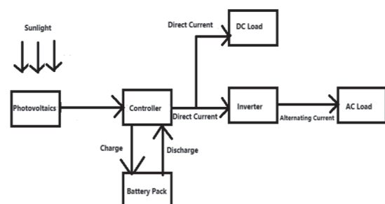
Fig. 3. Basic structure of photovoltaic power generation system (Picture credit: Original)
