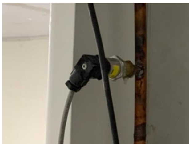
Fig. 4. The Gems Sensors 3100 series are used to measure refrigerant pressure intrusively.
