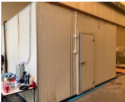
Fig. 2. Test chamber constituted from 4-inch PU panels.
