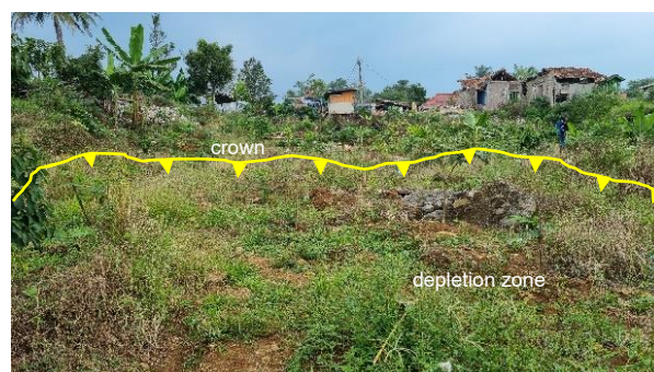
Fig. 7. Rawacina landslide showing the crown, a gentle slope and the undulating morphology of the depletion zone.
