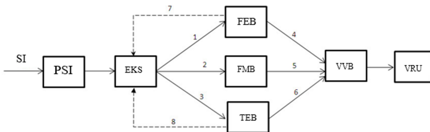
Fig. 1. Diagram of the solar optocoupler device, 1, 2, 3 – optoelectronic circuits, 4, 5, 6 – electrical connecting circuits, 7, 8 – electrical circuits for feedback, VVB – high-voltage unit, FEB – photovoltaic unit, TEB – thermoelectric block, FMB – photo-magnetic-electric block, PSI – solar radiation receiver, EX – electronic switching system, ASU – output operating device with dielectric load, SI – solar radiation, OBS – feedback.
