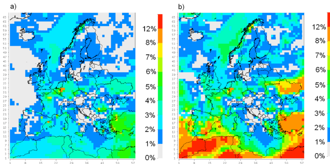
Fig. 2. Ratio of oxidized mercury ( \text{Hg}^{2+} = \sum \text{GOM} + \text{Hg}_p ) to total mercury ( \text{Hg}_{\text{TOT}} = \sum \text{Hg}^0 + \text{Hg}^{2+} ) in an altitude of 250m to 400m in July 2009 using boundary conditions from different global models a) GLEMOS, b) ECHMERIT. (preliminary results)
