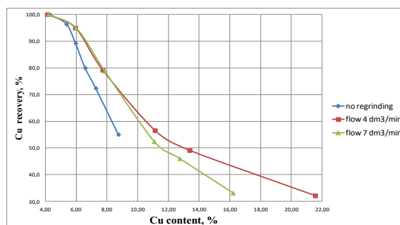
Fig. 7. Flotation results of the reground in MM carbonate middlings from Rudna Concentrator.
