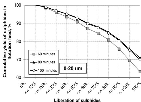
Fig. 7. Liberation of sulphide particles in the size range of 0–20 \mu\text{m} in flotation feed.
