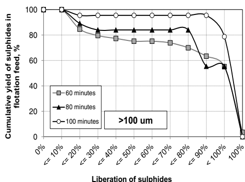
Fig. 8. Liberation of sulphide particles in the size range of >100 \mu\text{m} in flotation feed.
