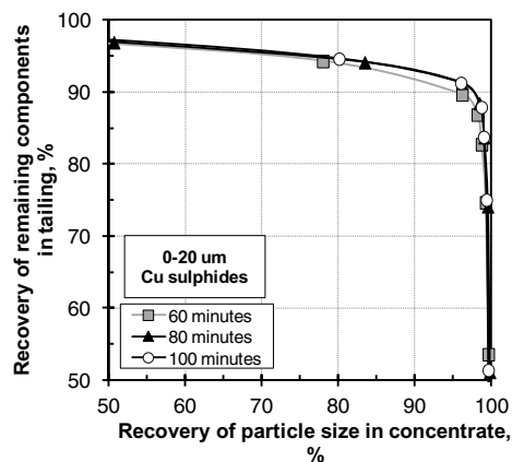
Fig. 9. A recovery of copper sulphides in concentrate vs. recovery of remaining components in tailing in size range of 0–20 \mu\text{m} obtained after 60, 80 and 100 minutes of milling.
