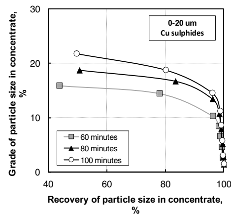
Fig. 10. Copper sulphides grade vs. recovery in size range of 0–20 \mu\text{m} obtained after 60, 80 and 100 minutes of milling.
