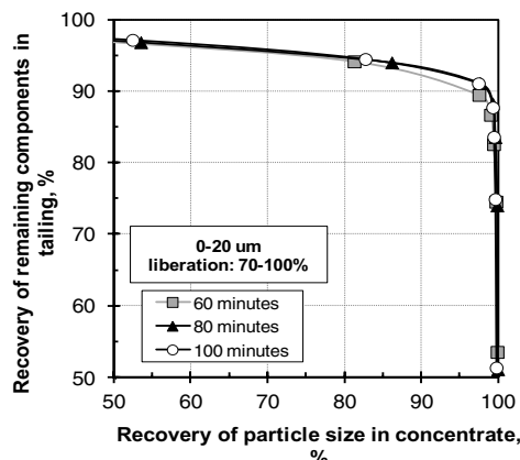
Fig. 13. A recovery of sulphides vs. recovery of remaining components in tailing in size range of 0–20 um liberated in 70–100% (free particles) obtained after 60, 80 and 100 minutes of milling.
