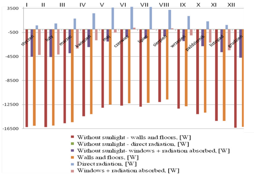
Fig. 4. Monthly variation of heat gains by buildings structure.
