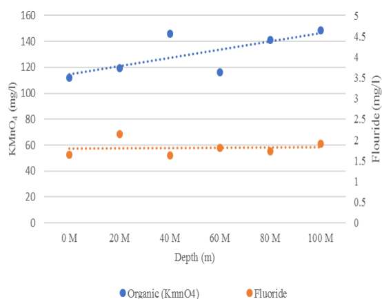
Fig. 4. Chemical Properties Organic and Flouride
