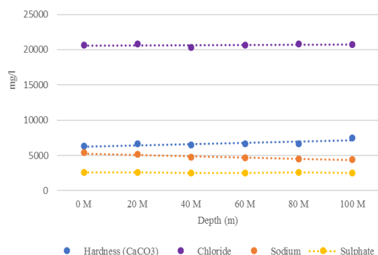
Figure 5. Chemical Properties ; Hardness, Chloride, Sodium and Sulphate
