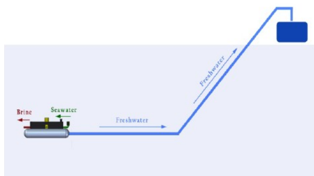
Fig. 2. Deep sea reverse Osmosis scheme[19]
