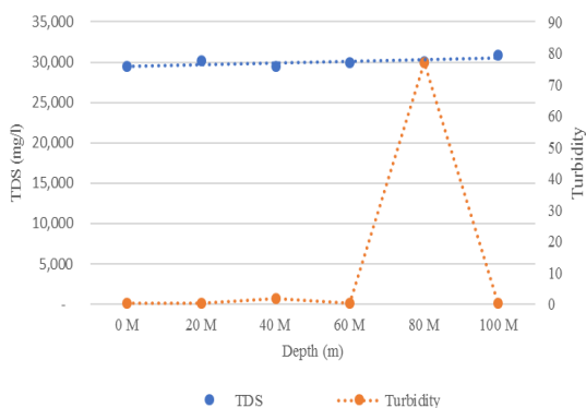
Fig. 3. Physical Properties TDS and Turbidity
