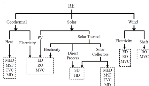
Fig. 1. Possible technological combinations of the main renewable energies and desalination methods[18]
