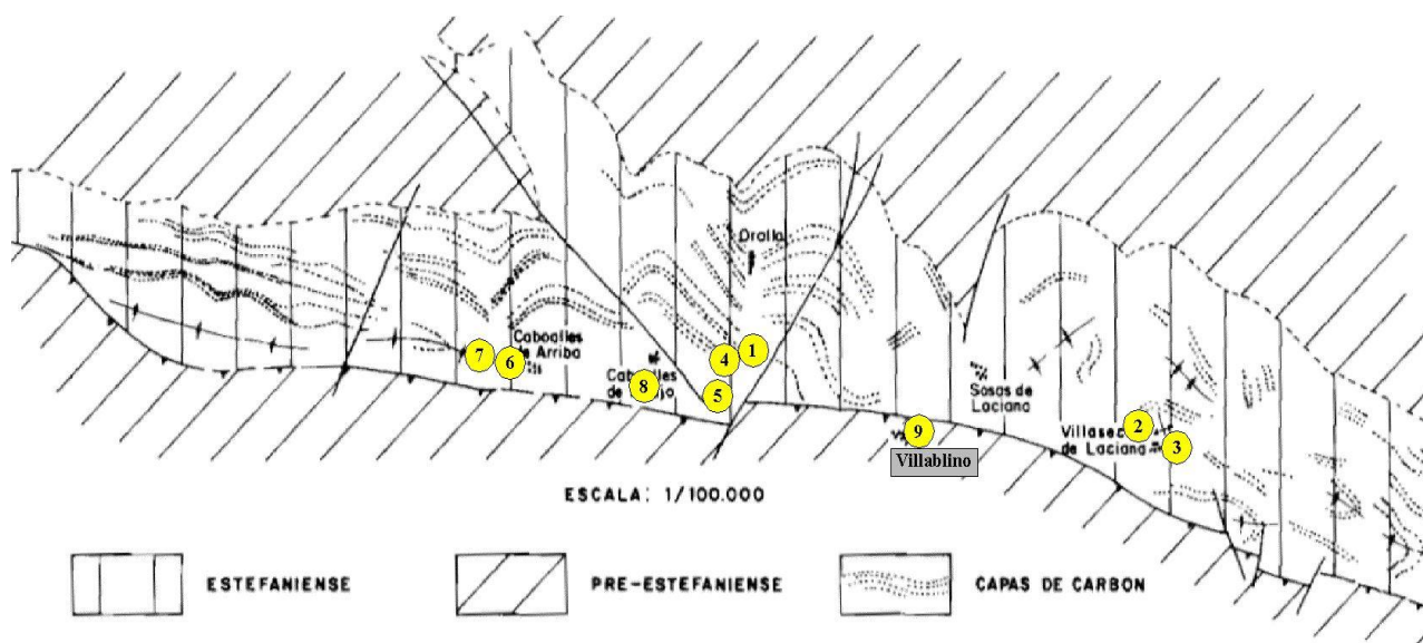
Figure 1. Geological scheme of Laciaña mining area and sampling points location [12].
