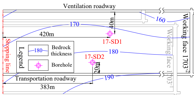
Fig. 3. Sketch map of observation borehole location
