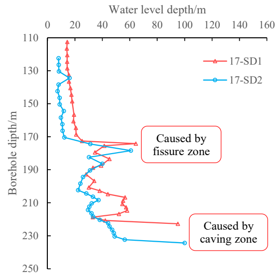
Fig. 4. Water level variation of boreholes
