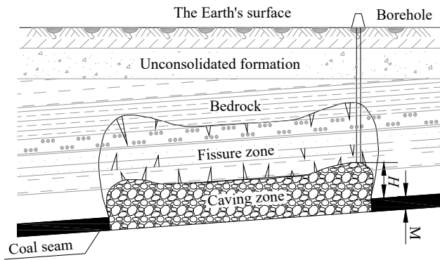
Fig. 2. Diagrammatic sketch of caving zone observation
