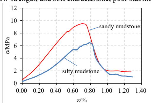
Fig. 1. Stress-strain curve of uniaxial compressive strength
