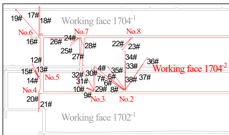
Figure 6. Boreholes in the area near open-off cut
