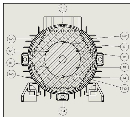
Figure 2. Thermocouple placement.
