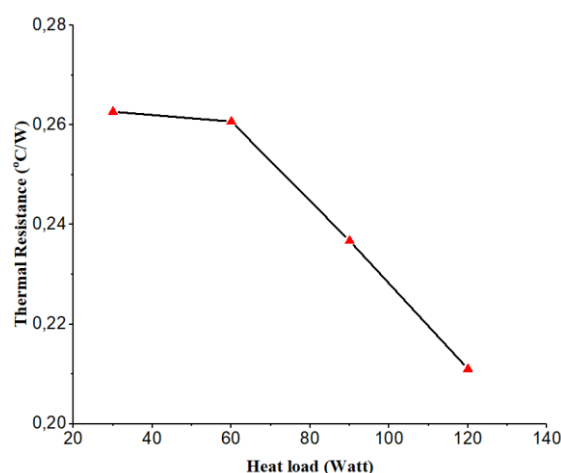
Figure 7. The thermal resistance of PHP.
