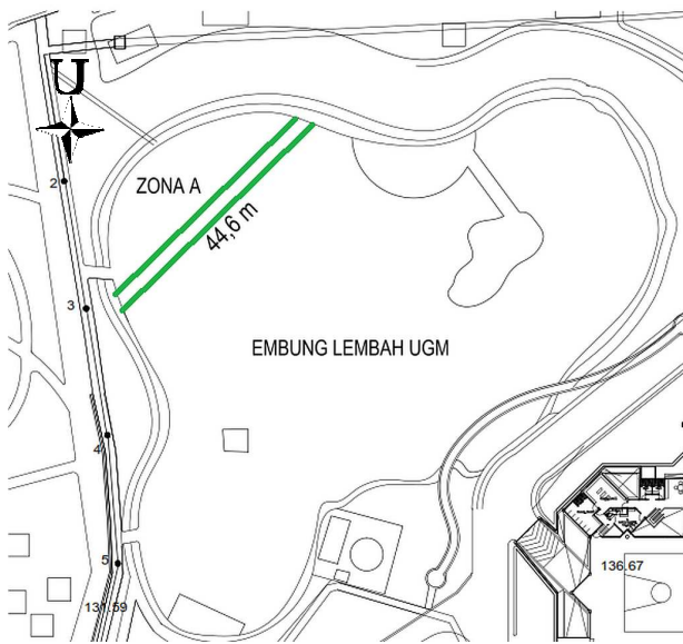
Fig 5. Location of Horizontal-flow Roughing Filter design.
