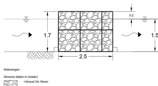
Fig. 7. HRF Cross Section.
