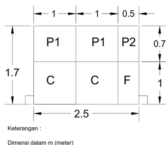
Fig. 6. Location of Horizontal-flow Roughing Filter design
