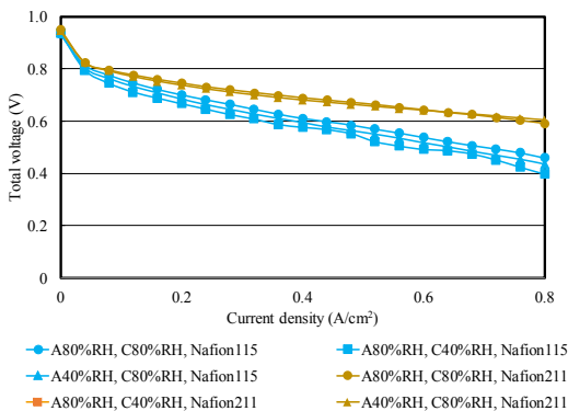
Fig. 8. Polarization curves of two different PEMs under various relative humidity conditions in the case of T_{ini} = 90\text{ }^{\circ}\text{C} .
