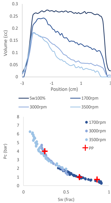
Figure 2. Results for primary drainage applied on the Richmond sample. NMR profiles (top), resulting Pc curve (bottom).
