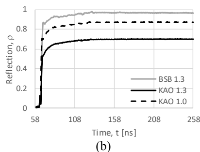
Fig. 2. Waveform for samples of KAO and BSB (a) 10ns window and (b) 200ns window
