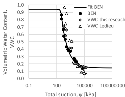
Fig. 12. Soil Water Retention curve for BEN samples
