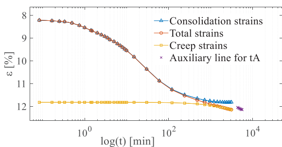
Fig. 7. Oedometer step filtered in ANACONDA.
