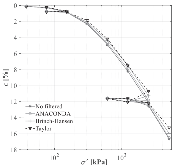
Fig. 13. Different separation of strains methods on Test03.
