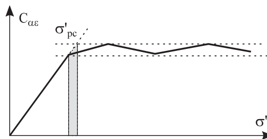
Fig. 8. Akai uses C_{\alpha\varepsilon} to determine preconsolidation stress.
