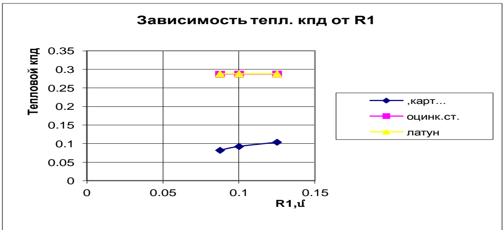
Fig.2. The change of the thermal efficiency of three-pipe recuperator, depending on R_1 = c \frac{d_{св.в.}}{2} (under canonical arrangement of pipes for air removal), pipe dimensions and used
