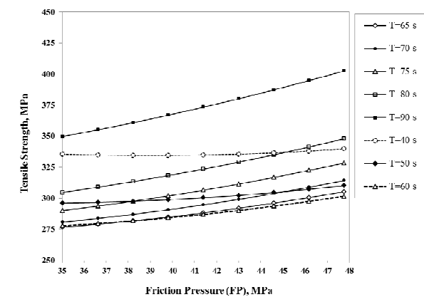
Fig. 6. Effect of friction pressure and friction time on tensile strength
