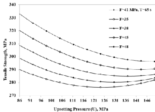
Fig. 7. Effect of upsetting pressure and friction pressure on tensile strength
