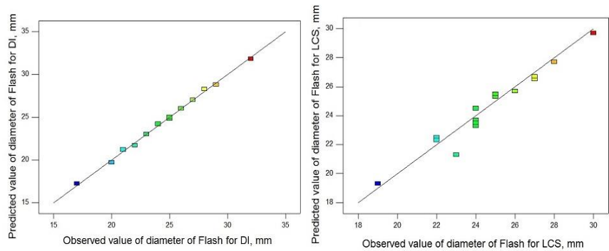
Fig. 1. Predicted value of flash diameter vs. observed value of flash diameter
