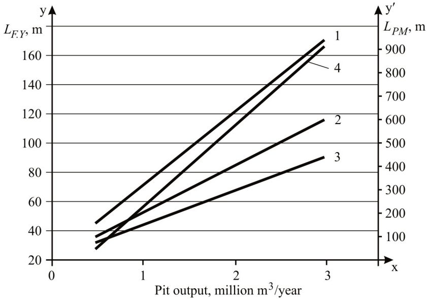
Fig. 2. The dependence of the pit mining front ( L_{F.Y} ) and face cut movement ( L_{P.M} ) relatively to pit mining front on the production capacity: 1, 2, 3 – cut width ( A_3 ) – 20, 40, 60 m, accordingly; 4 – pit mining front movement ( L_{F.Y} ).
