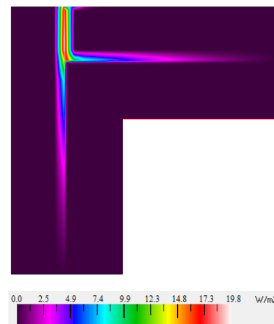
Fig. 5. The intensity of heat flow through the wall corner insulated with aluminium foil faced PIR, without PU glue
