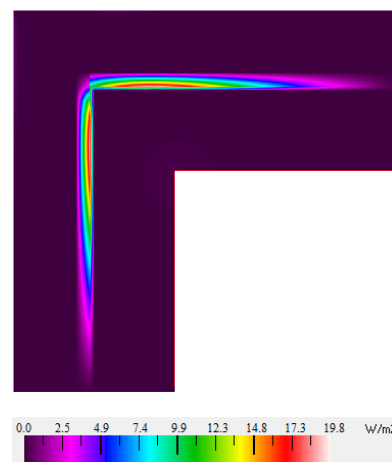
Fig. 6. The intensity of heat flow through the wall corner insulated with aluminium foil faced PIR, without aluminium foil in the joint
