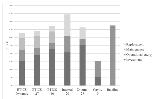
Fig. 7. NPV wall constructions after 60 years.
