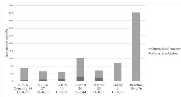
Fig. 3. Environmental score of wall constructions after 60 years.
