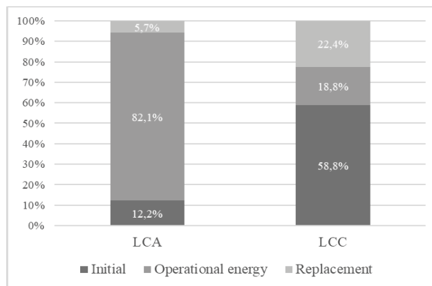
Fig. 6. Contribution life cycle phases.
