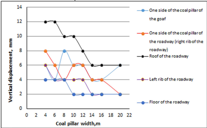
Fig. 6. Vertical displacement of the coal pillar and roadway under different coal pillar widths.
