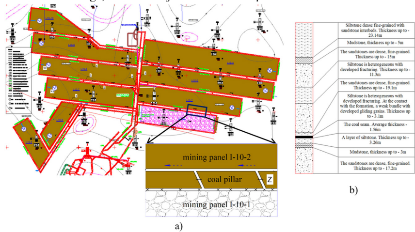
Fig. 1. Layout and roof lithology of the working faces of the coal seam 10: a) layout of the working faces; b) lithological profile.
