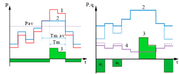
Fig. 2. Daily power and specific fuel consumption profiles: a - load power profiles (1), generator (2), ESS (3); b - power profiles and specific fuel consumption (4).
