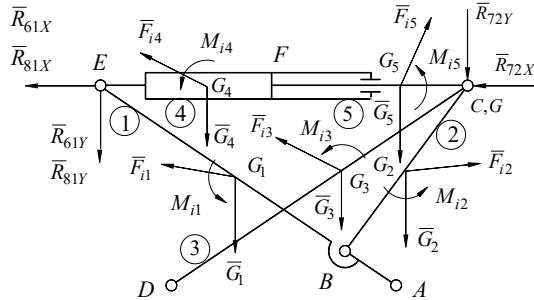
Fig. 5. The motor tetrad RRR-Ta-RRR(1,2,3,4,5) . Highlighting the forces and moments acting on the elements of the structural group
