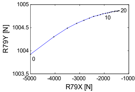
Fig. 9. The hodograph of reactions in coupling L
