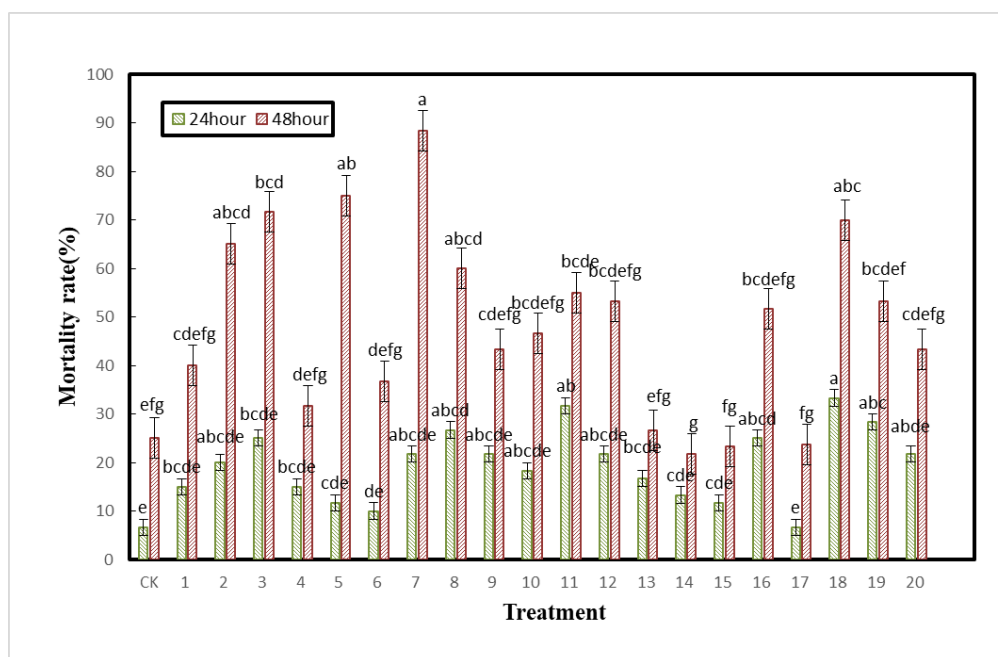
Fig. 1 Effects of E. bromicola on the insecticidal rate of R. padi
