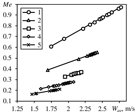
Fig. 3. Dependence of the Merkel number in the mean-flow velocity of air at the different wetting densities q_L , kg/(m 2 ·s): 1 – 3.25; 2 – 4.97; 3 – 6.70; 4 – 8.42; 5 – 10.15.
