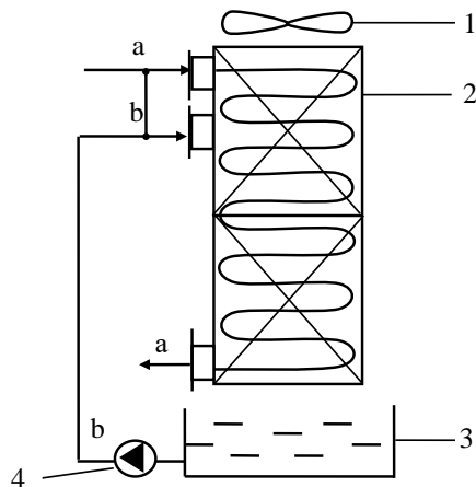
Fig. 1. Schematic diagram of the non-chemical cooling tower with the inclined-corrugated contact elements: 1 – fan; 2 – filler unit; 3 – water-collecting pond; 4 – pump.
