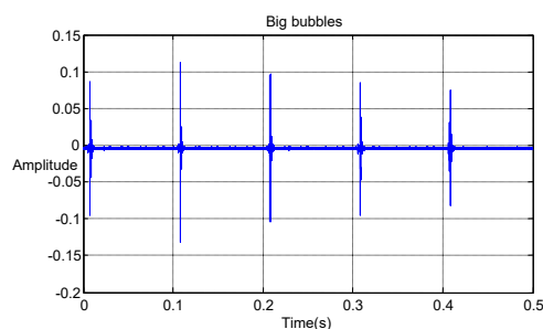
Fig.5. Acoustic in big bubbles
