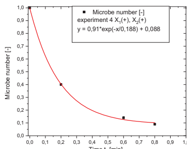
Fig. 3 Graph for the reduction of the microbial number during cavitation processing in an dimensionless form
