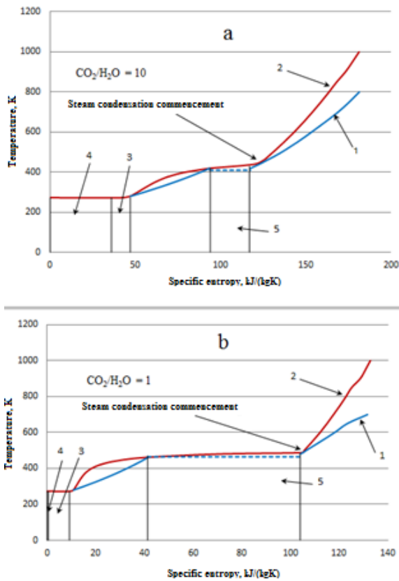
Fig. 8. The cooling process of the spent working fluid in T-S coordinates: 1 - line for heating the components of the working fluid before feeding into the combustion chamber; 2 – line for cooling of the spent working fluid; 3 - heat for warming up fuel and oxygen to the temperature of CO 2 condensation; 4 – heat, removed into the environment; 5 – heat, delivered to the heating system.
