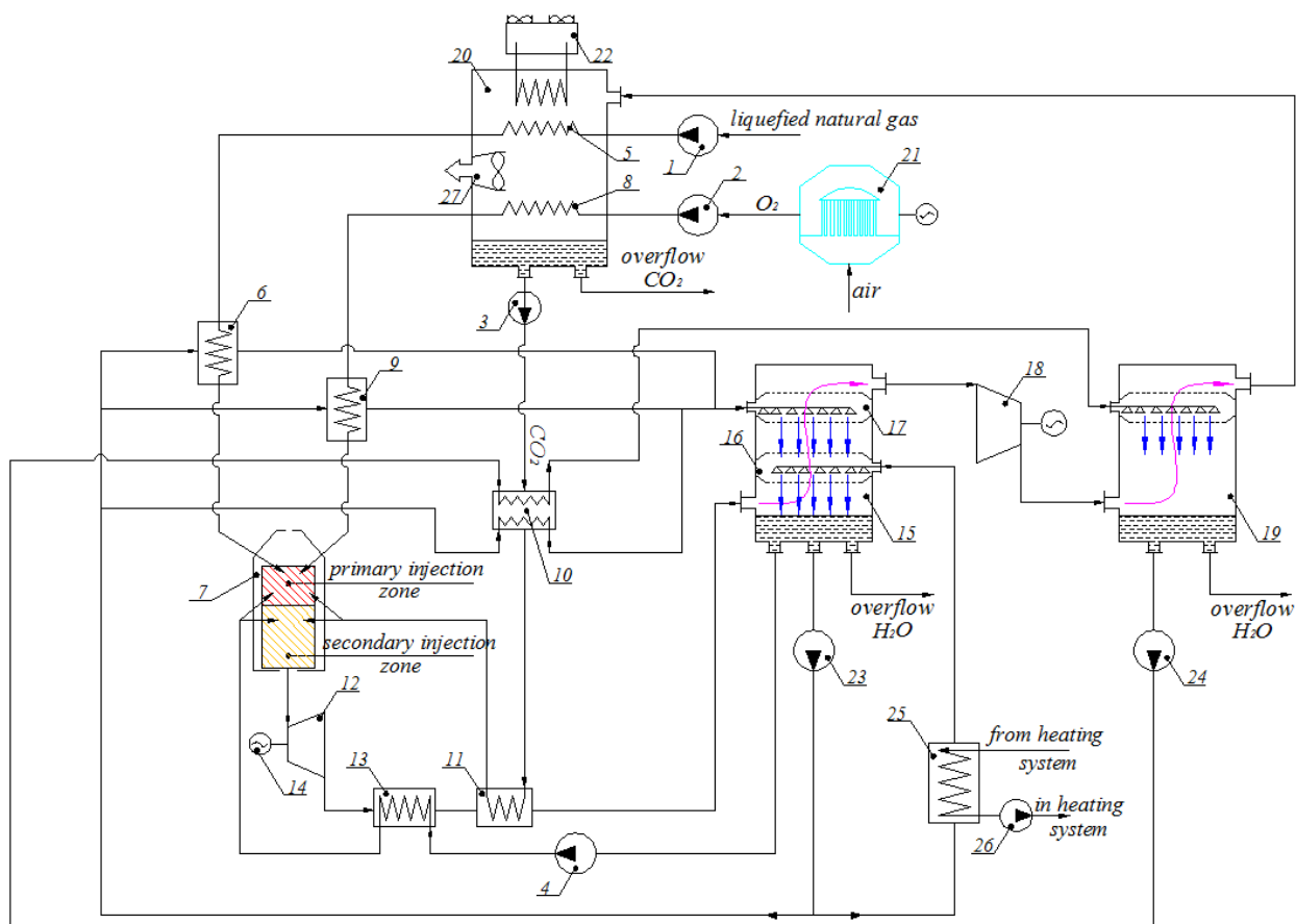
Fig. 1. Compressorless combined cycle gas turbine unit schematic.
