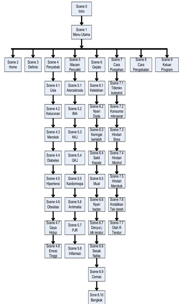
Fig. 1. Navigation Structure.
