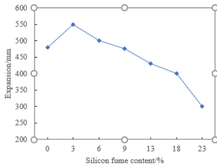
Fig1. The influence of silica fume content on HPC expansion.
