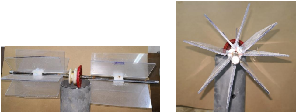
Fig. 10. The axis with 8 rectangular paddles from the optimized submersible module.
