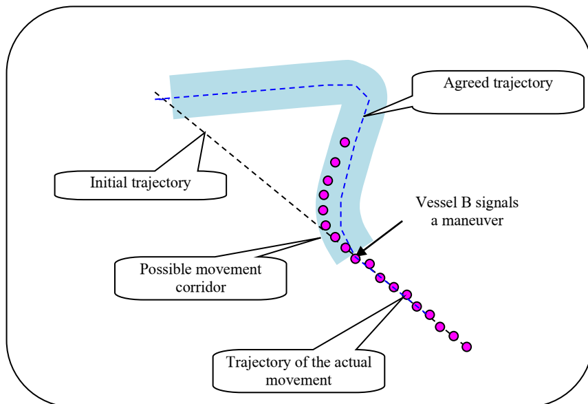
Fig. 2. False triggering of the detector of violation of agreements by agent of vessel A.
