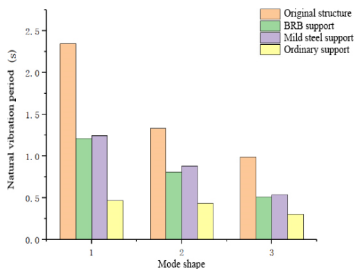
Fig.2. Comparison chart of natural vibration period of shock-absorbing structure
