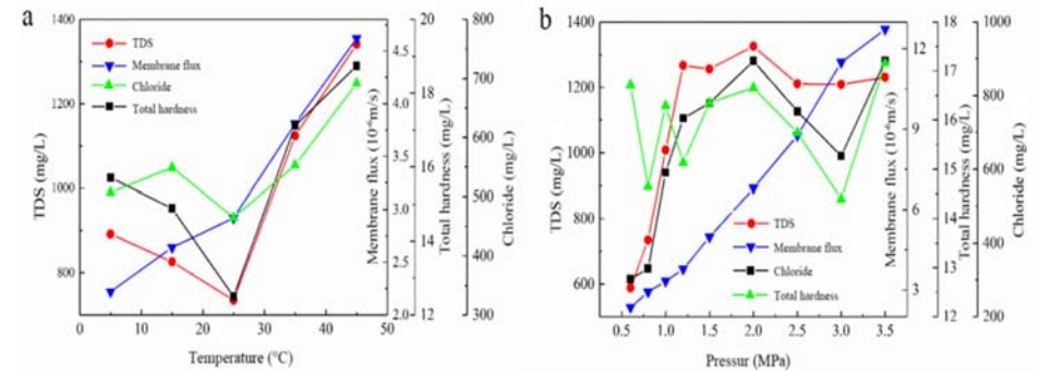
Fig. 3. Filtration effect of NF90 membrane at different operating (a) temperature and (b) pressure.
