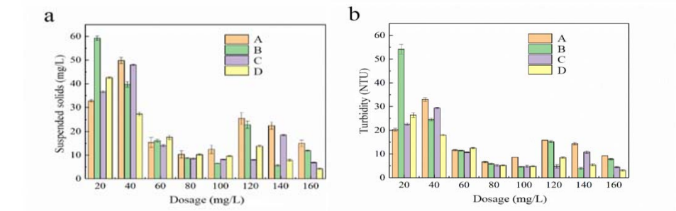
Fig. 2. Change of effluent (a) suspended solids and (b) turbidity at different dosage of coagulant.
