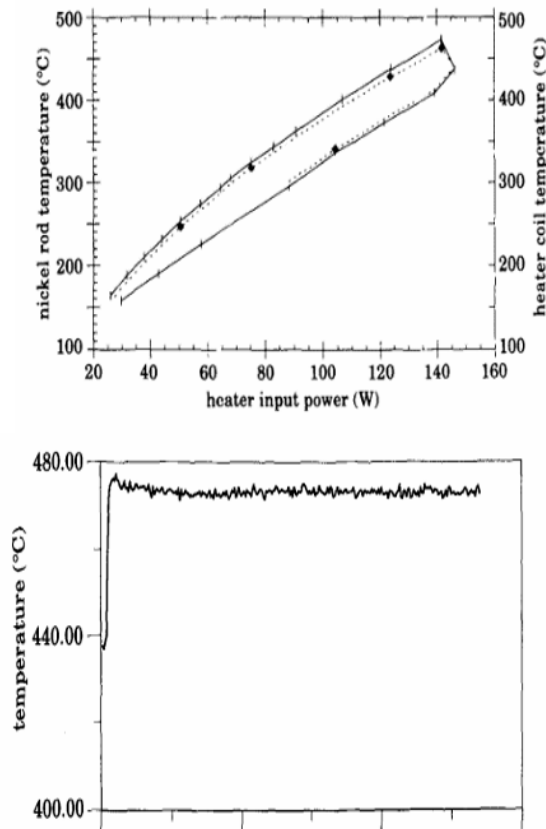
Fig.1 The abnormal exothermic phenomenon of the experiment of S. Focardietal.
