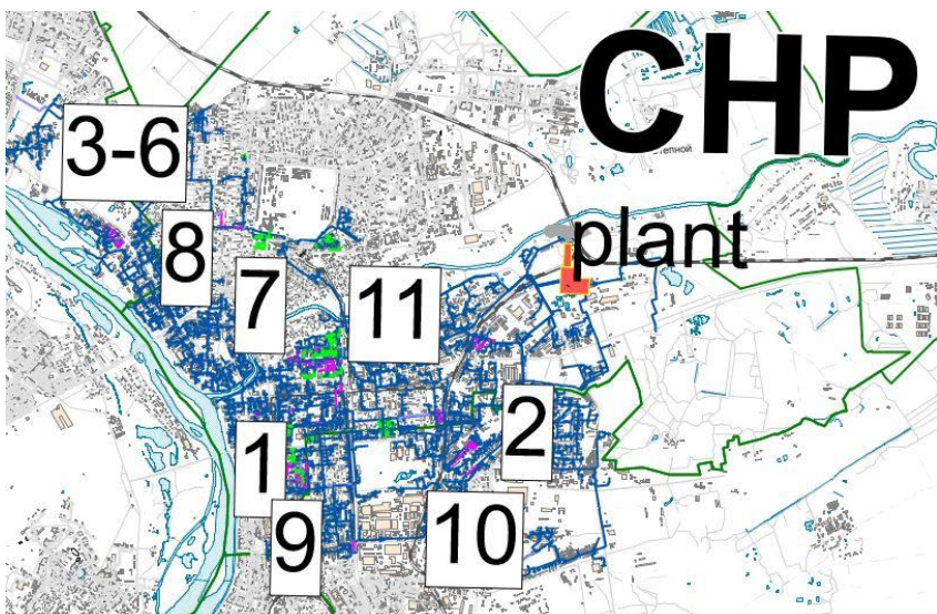
Fig. 1. DH system layout with buildings labels.
