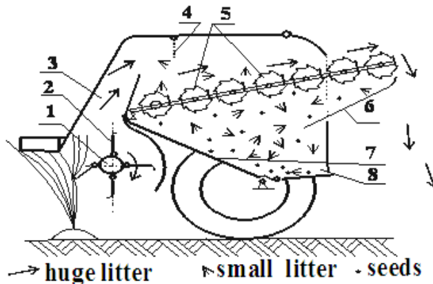
Fig. 3. Seed picker diagram
