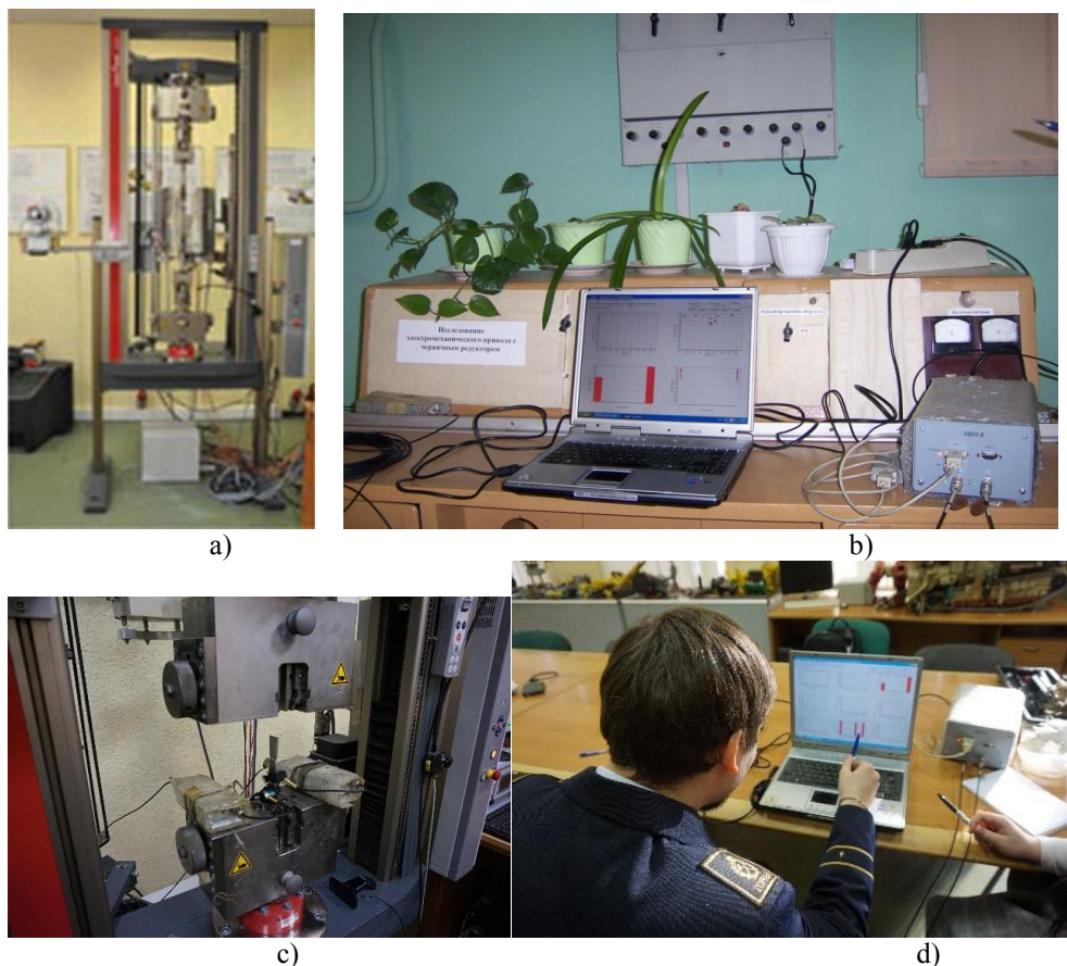
Fig. 3. Equipment used for the experiment: (a) universal testing machine Zwick / Roell Z100; (b) acoustic emission equipment, (c) acoustic emission transducers located on the sample, (c) acoustic emission registration process.
