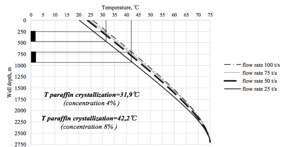
Fig. 3. Temperature distribution over the depth of the well.
