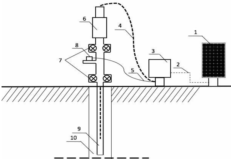
Fig. 4. Composition of the electric heating well complex.
