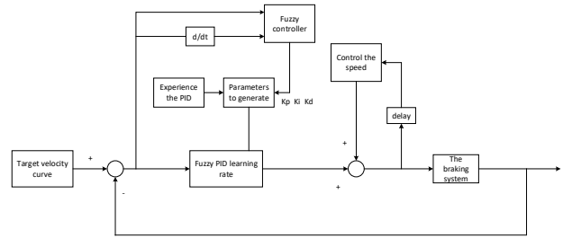
Fig. 3. Fuzzy PID learning control diagram
