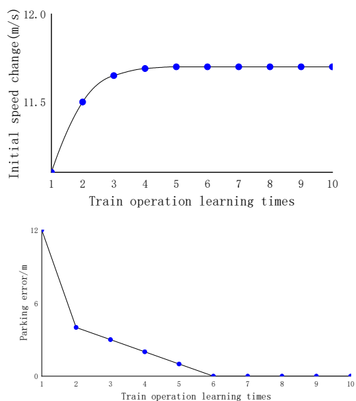
Fig. 5. Initial speed adjustment
