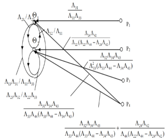
Fig.5. After being excluded \theta_3 from the graph
