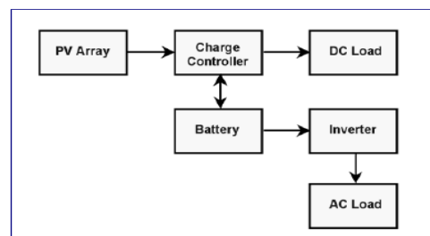
fig1: PHOTOVOLTAIC SYSTEMS –Standalone System
