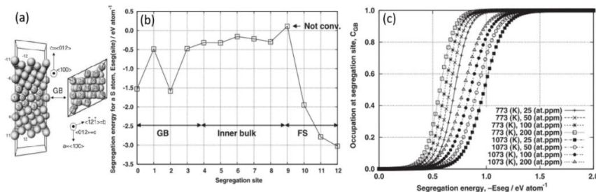
Fig. 2. The segregation of S atoms at Ni inner grain, grain boundary (Ni \Sigma 5 (012) [100]) and surface [8] (a) grain boundary model of Ni \Sigma 5 (012) [100], (b) segregation energy corresponding to S atoms at different positions in grain boundary of Ni \Sigma 5 (012) [100], (c) plots of McLean’s equation for some segregation conditions (ageing temperature and bulk impurity concentration).
