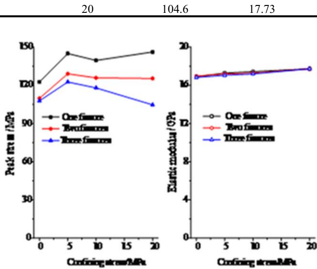
Fig. 3. the relationship between mechanical parameters and confining stress
