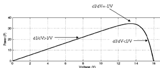
Fig. 6. P-V characteristics for P&O Algorithm.
